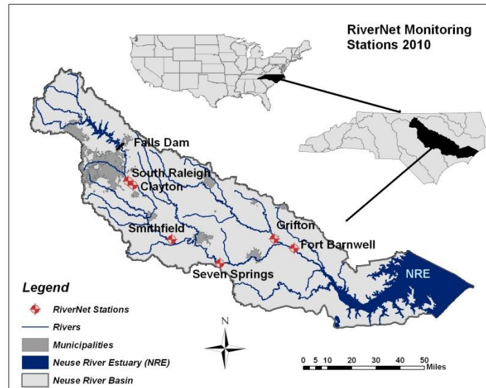
Figure 1. The RiverNet monitoring network with stations located above and below the Neuse River Waste Water Treatment Plant (NRWWTP). Due to continued budget restrictions, two lower basins stations were temporarily closed down at Hookerton and Bear Creek.
