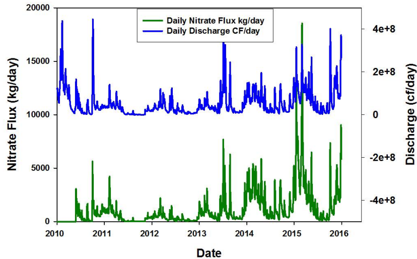
Figure 5. Nutrient flux at the Tomahawk River in the Cape Fear Basin.
