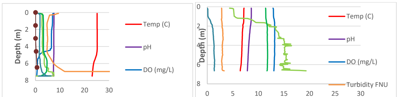
Figure 9. Water column profiles in Sept and January in Falls Lake at station H3 above the water treatment plant. Large bacterial mats have been found on the bottom of the lake and anoxia develops during summer
